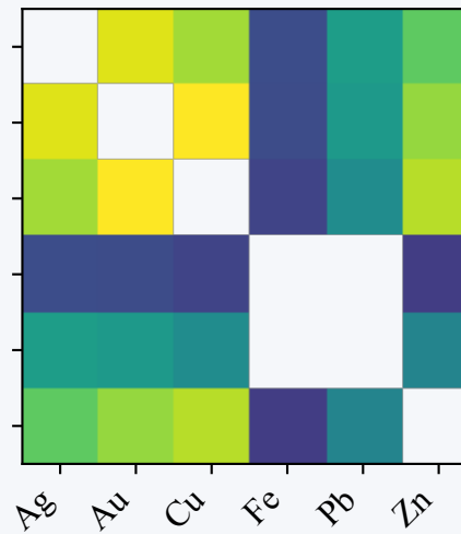
Close_Distance
