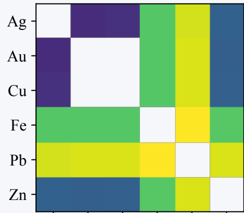
Euclidean
