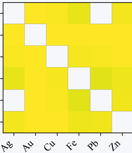
Correlation
