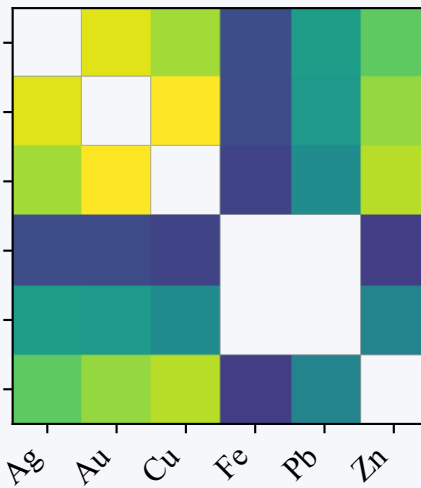
Hsim_Distance
