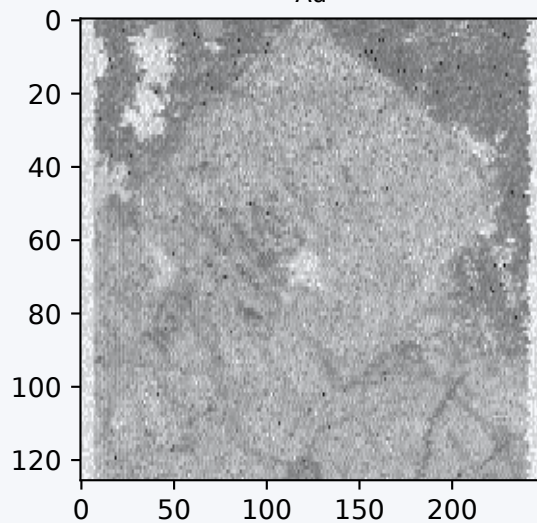
Pb
