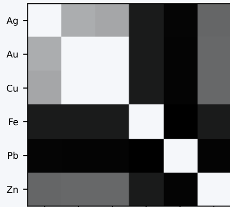
Euclidean
