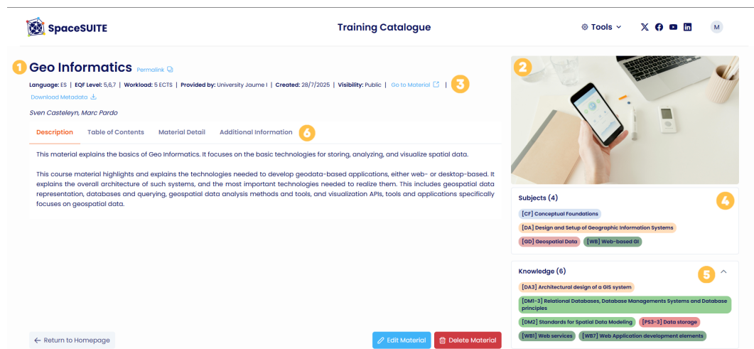
Figure 8: Training Catalogue detail view.
