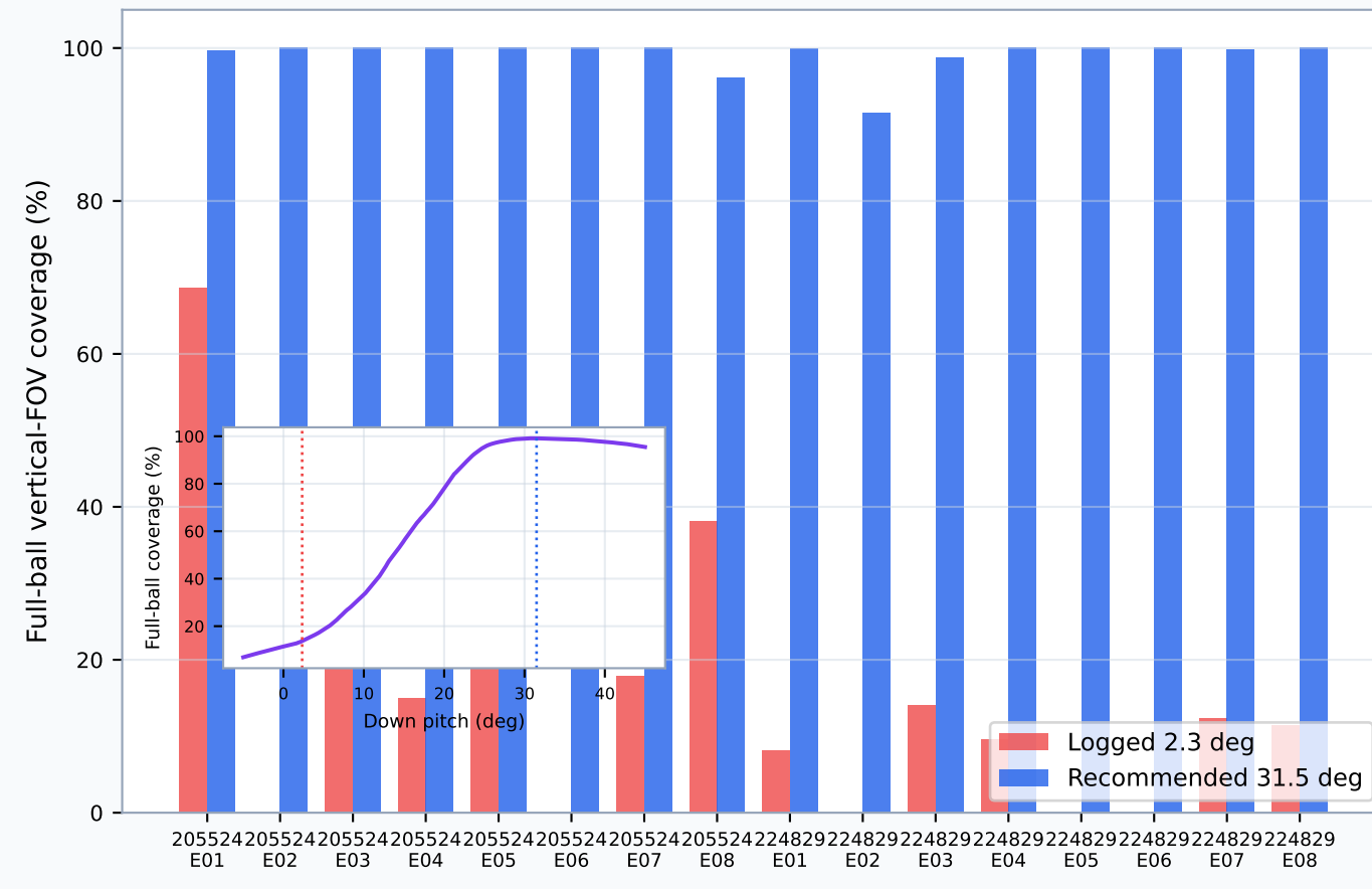
Conservative Coverage by Episode (entire 0.10 m-radius angular disk inside -7 deg to +52 deg)
