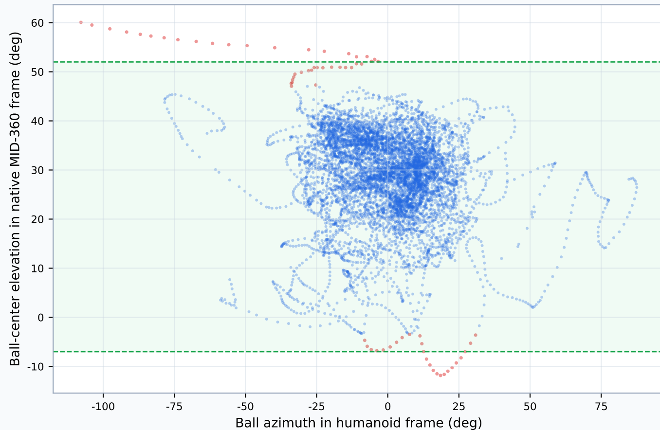
Recommended Mount inverted, 31.5 deg down; full-ball coverage=99.2%
