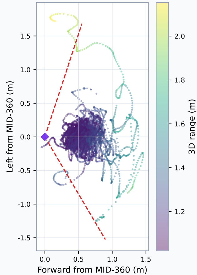
Top View: Trusted Ball Envelope 99% center azimuth: -59.5 deg to 71.9 deg
