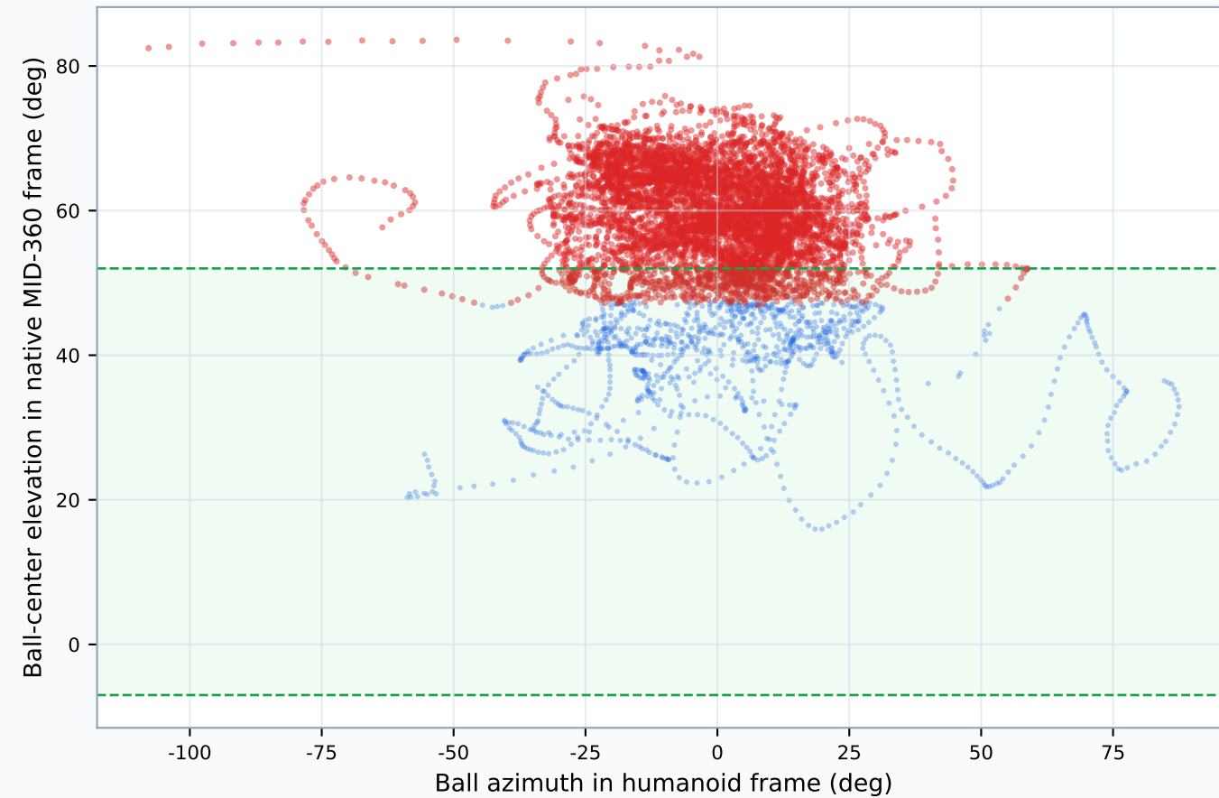
Logged Mount inverted, 2.3 deg down; full-ball coverage=13.8%
