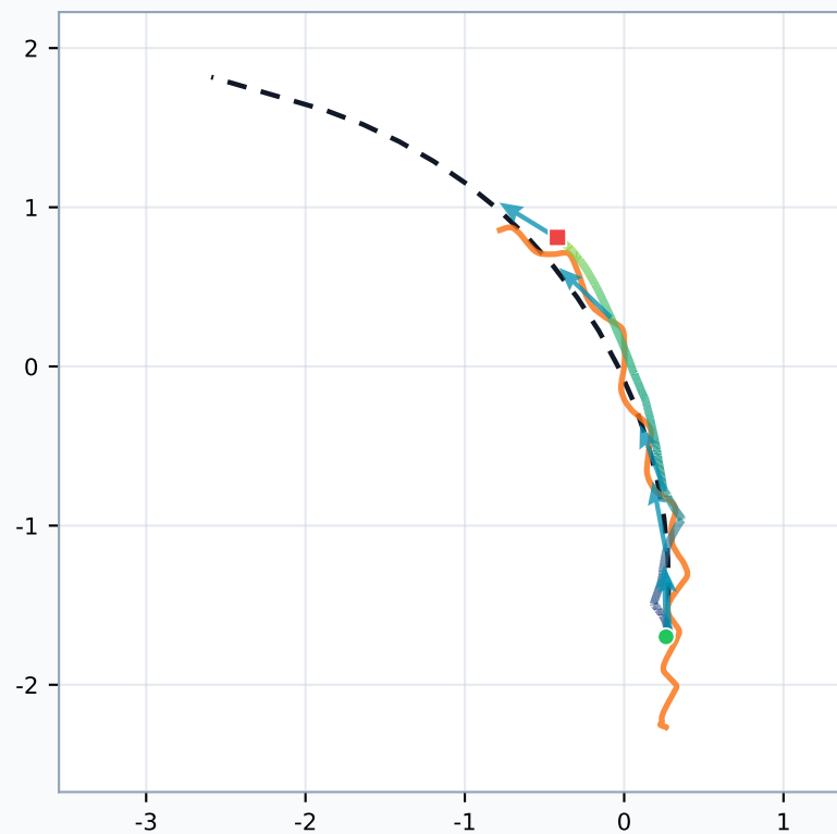
224829 / E02 · Best CT; truncate before mocap jump Ball CT mean/final: 0.075/0.140 m · Humanoid final: 0.071 m
