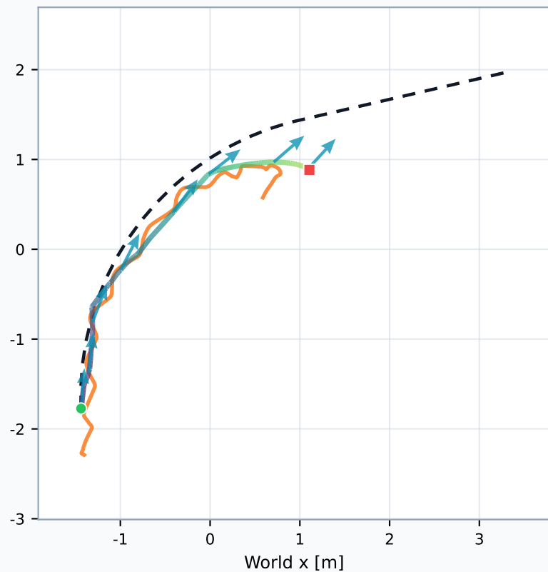
224829 / E05 · Ball and humanoid drift together Ball CT mean/final: 0.212/0.564 m · Humanoid final: 0.666 m
