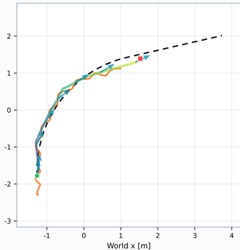
224829 / E08 · Low-CT reference Ball CT mean/final: 0.082/0.120 m · Humanoid final: 0.252 m
