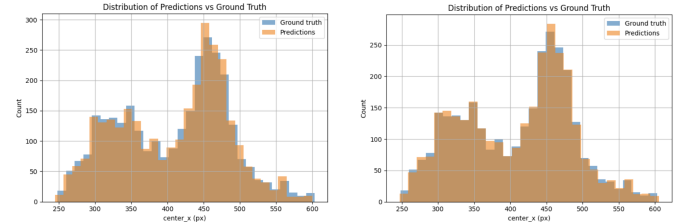
Figure 4.2: Predicted vs. ground-truth c_x distributions. Left: Base, Right: Enhanced.
