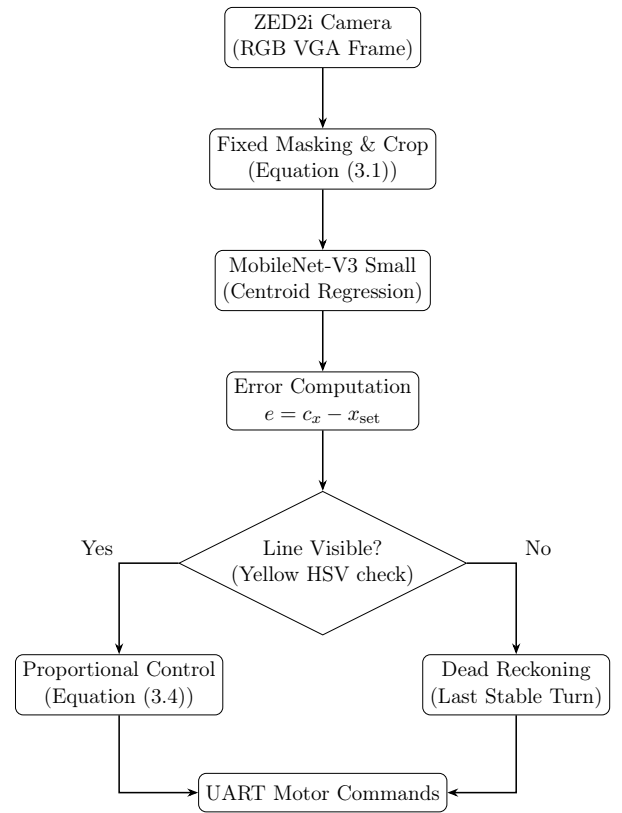
Figure 3.1: Overall Hybrid System Architecture.
