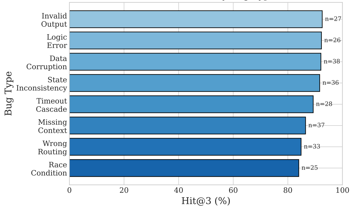
(b) Performance by Bug Type
