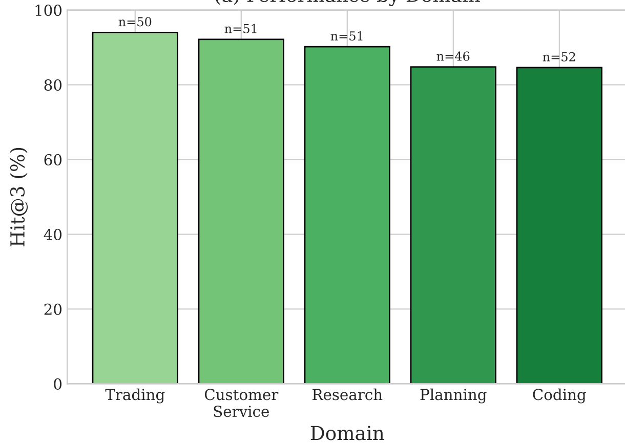
(a) Performance by Domain
