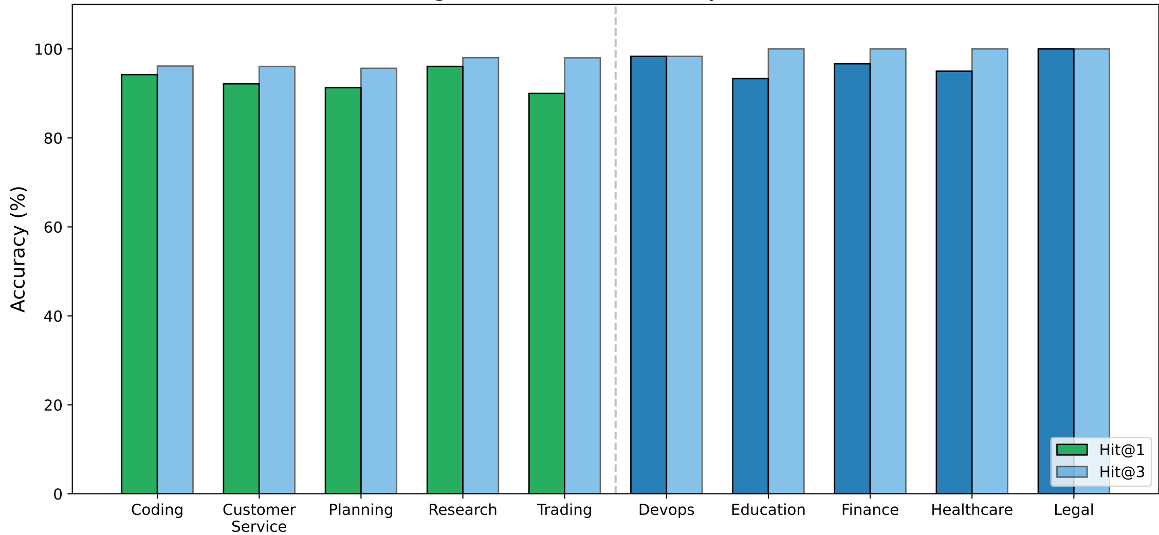
AgentTrace Performance by Domain
