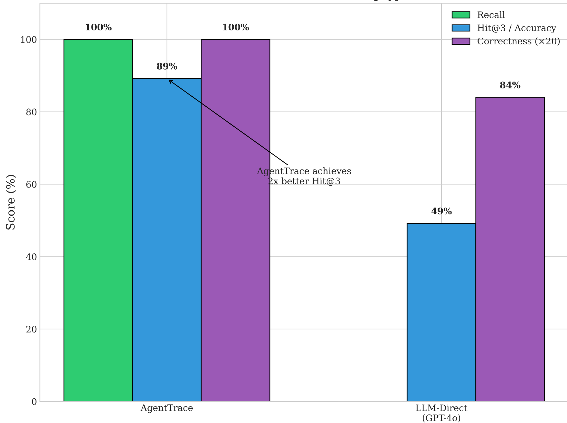
AgentTrace vs. LLM-Direct: Key Metrics Comparison (250 scenarios, 5 domains, 8 bug types)
