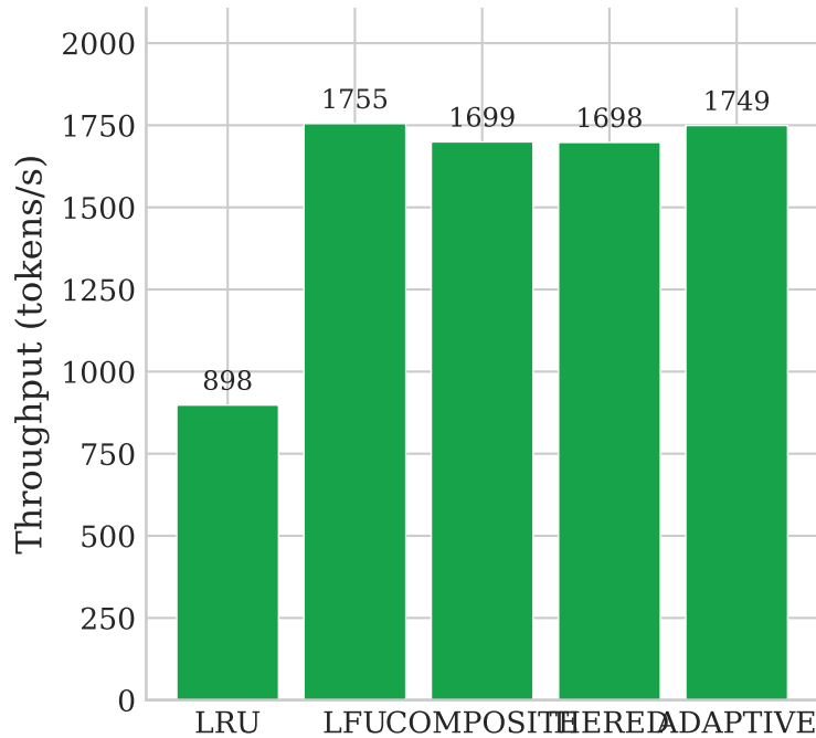
(b) Throughput by Policy
