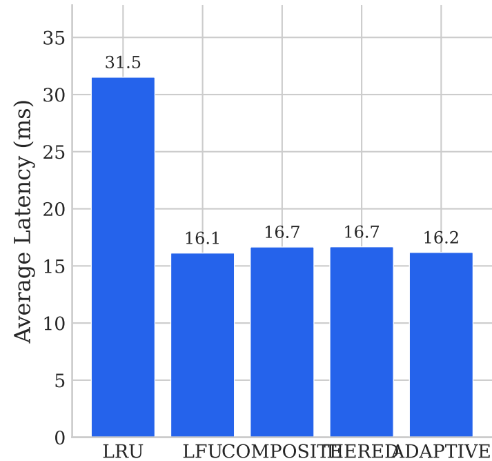
(a) Latency by Policy
