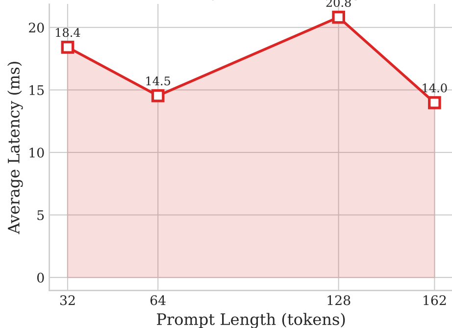
(b) Latency vs Prompt Length
