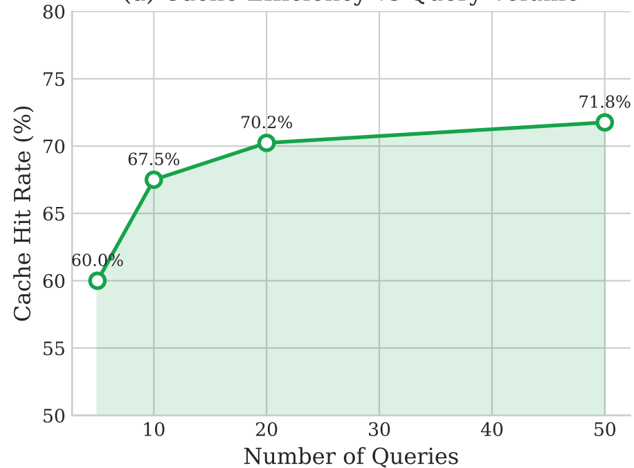
(a) Cache Efficiency vs Query Volume
