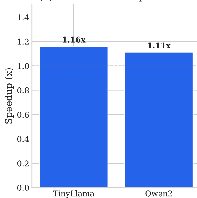
(b) Performance Improvement
