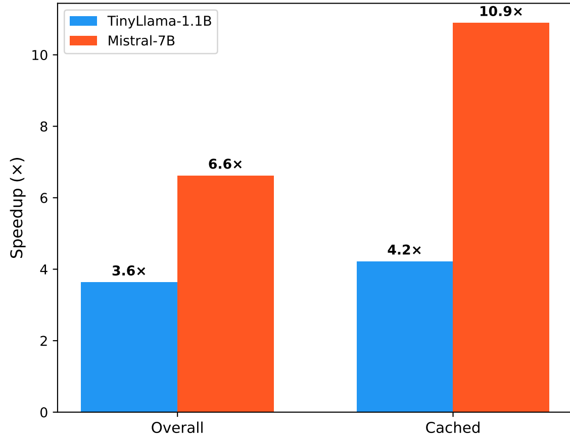
Code Completion Scenario
