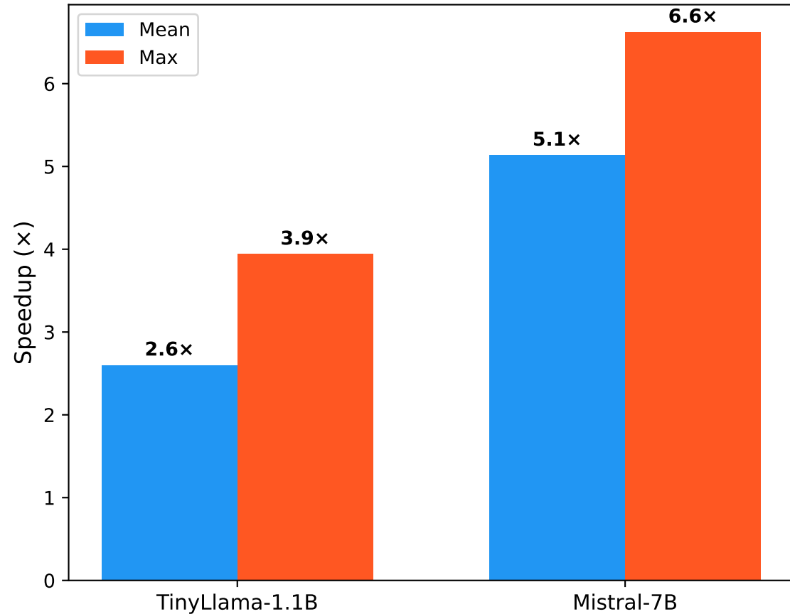
Model Comparison: Speedup
