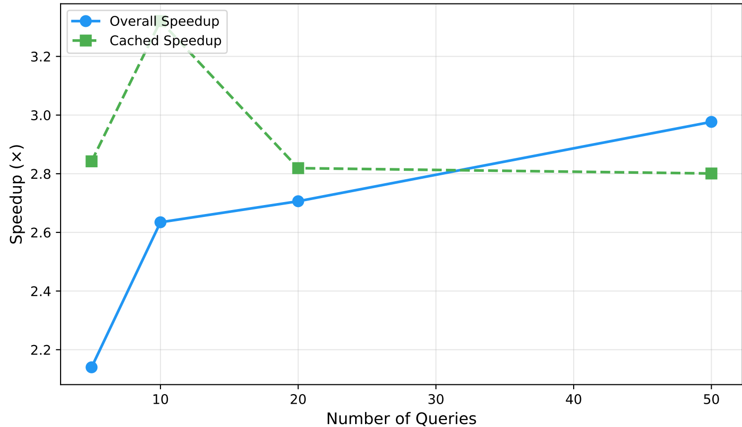
Speedup vs Query Count (Cache Amortization)
