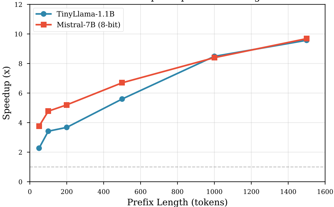
DeltaCache Speedup vs Prefix Length
