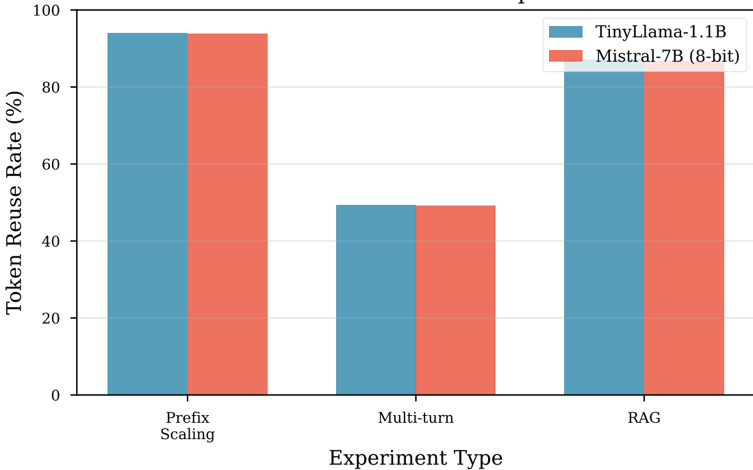
Token Reuse Rate Across Experiments
