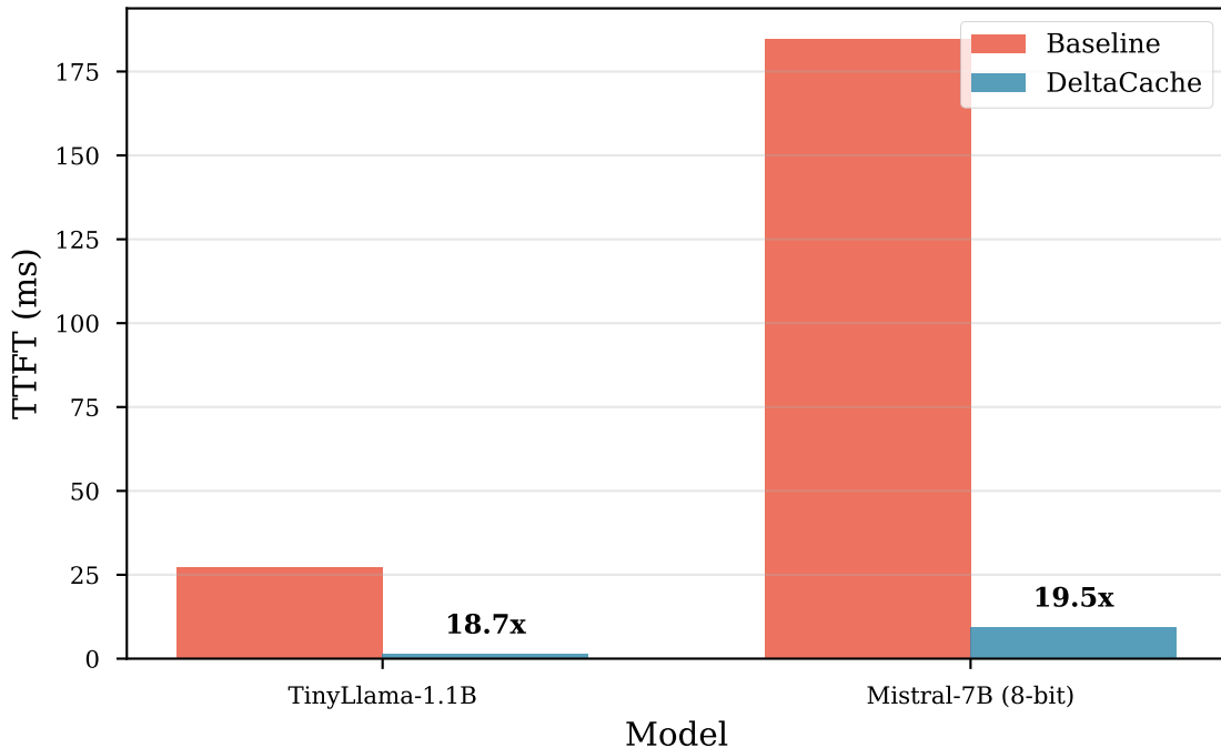
Time-to-First-Token Comparison (500 token prefix)
