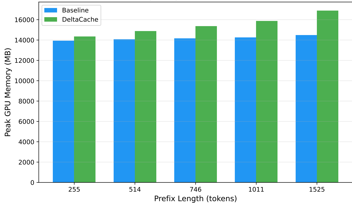
GPU Memory Usage: Baseline vs DeltaCache
