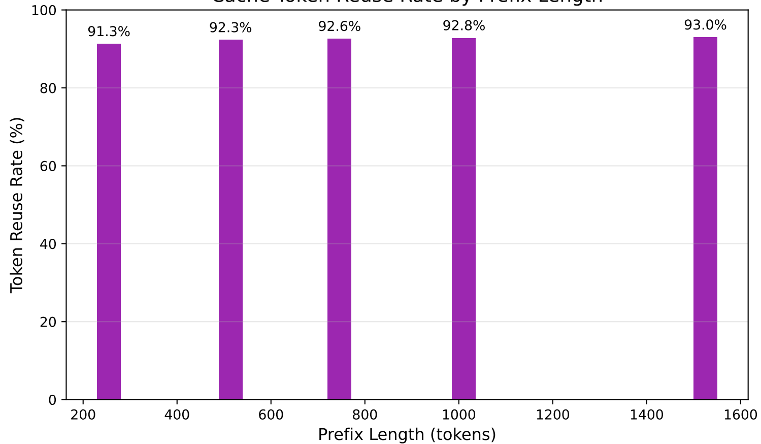
Cache Token Reuse Rate by Prefix Length
