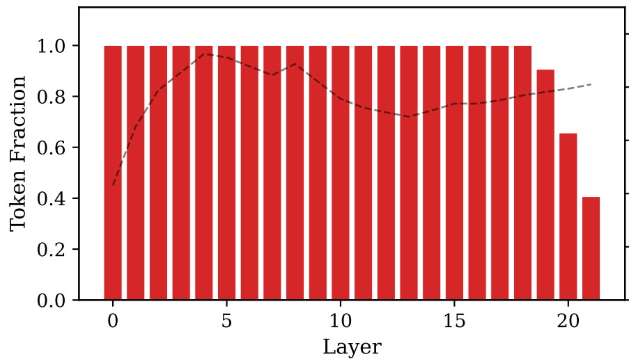
4× compression
