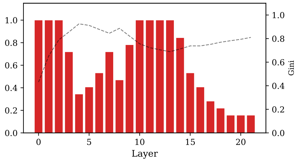
6× compression
