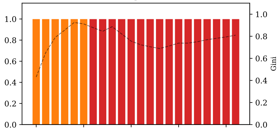
6× compression
