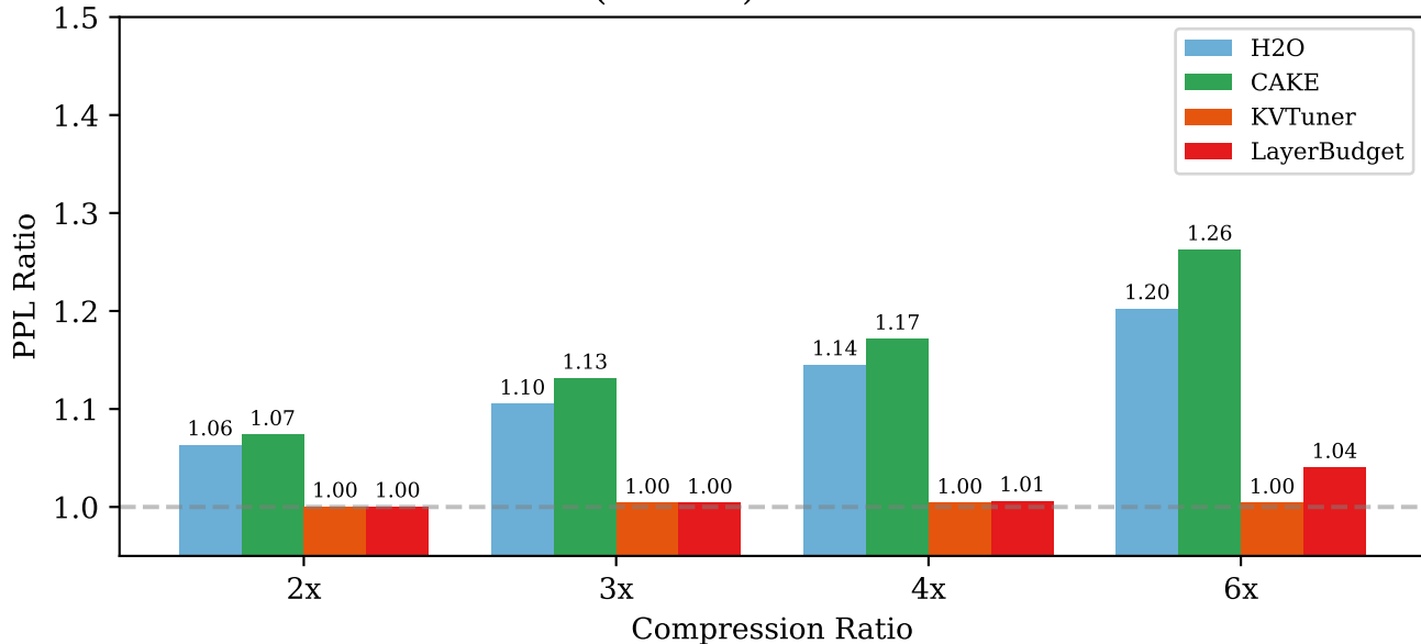
Mistral-7B (512 tok): Mean-Fill Evaluation
