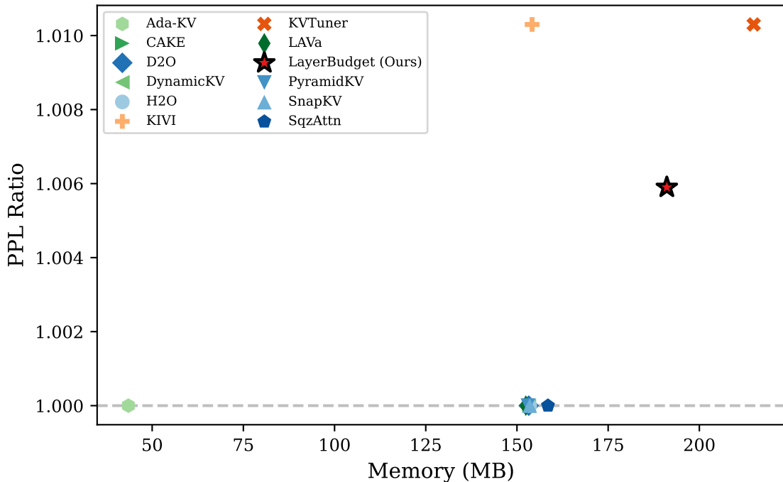
Llama-2-7B (2048 tok) @ 4x compression
