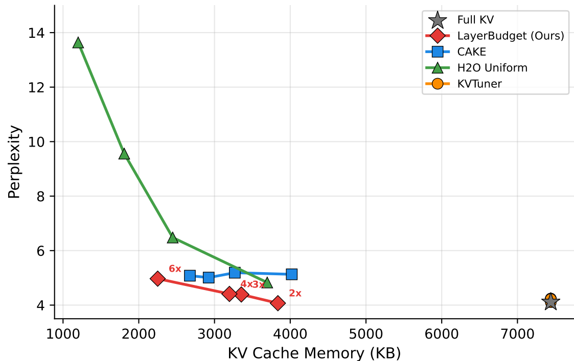
Mistral-7B (4-bit)
