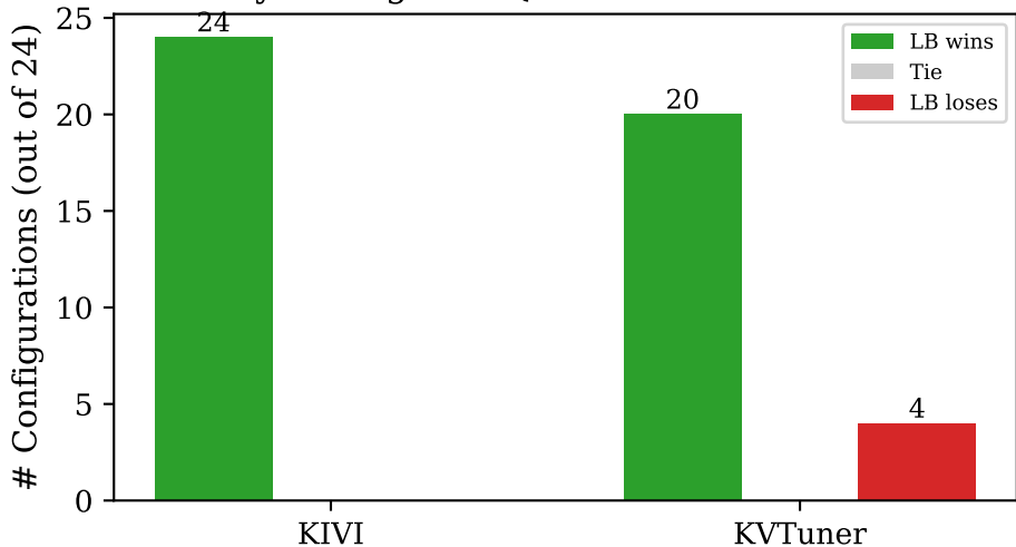
LayerBudget vs Quantization Baselines
