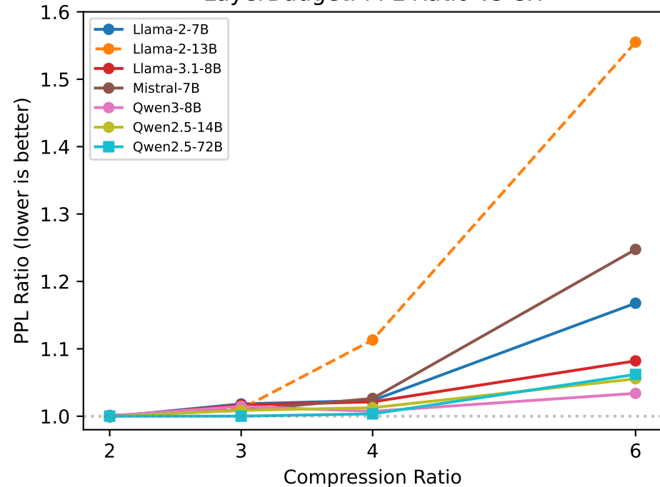
LayerBudget: PPL Ratio vs CR
