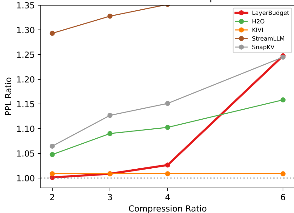
Mistral-7B: Method Comparison
