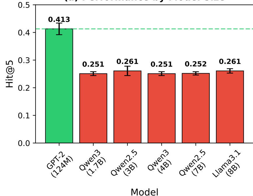
(a) Performance by Model Size
