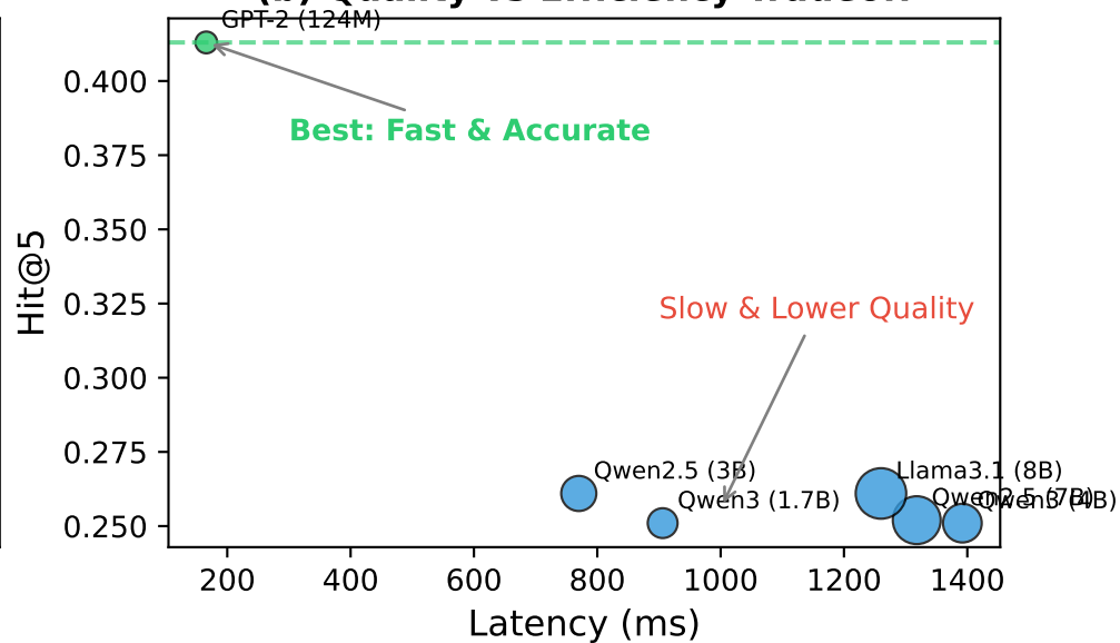
(b) Quality vs Efficiency Tradeoff
