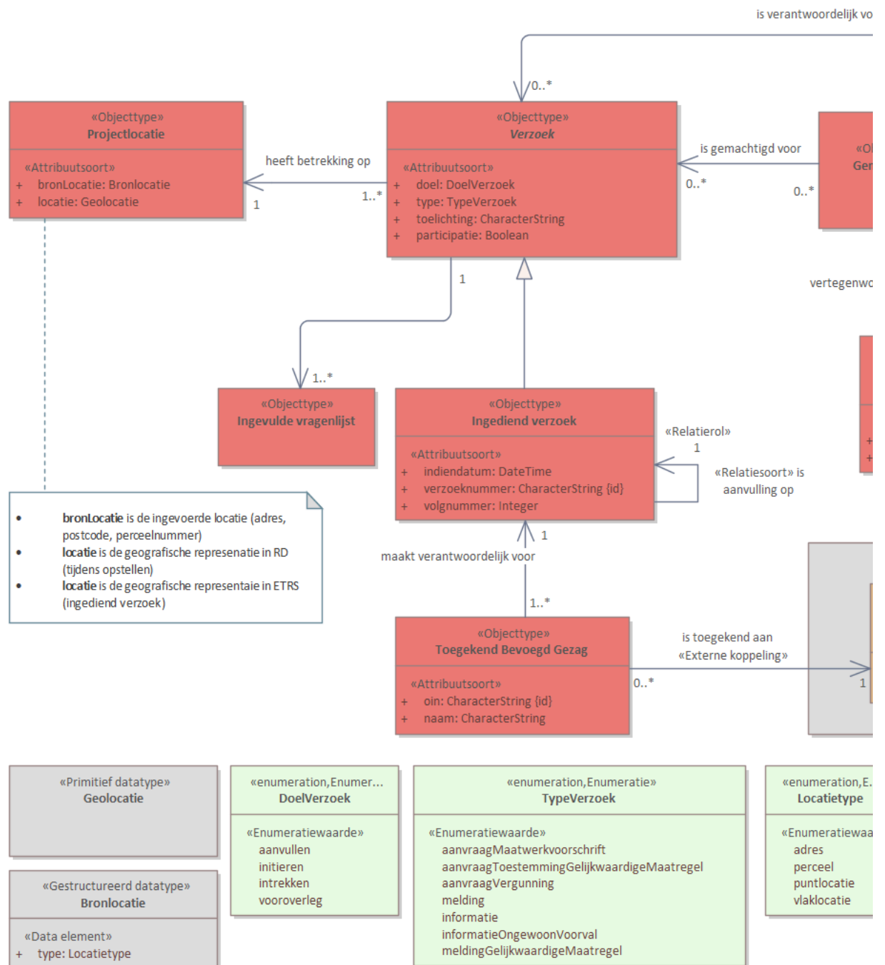
Figuur 3 – Diagram: CIM-AM Kern
