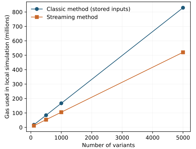
Figure 8: Gas used versus variant count for both calculation methods in the local simulation. The Streaming method used 35.4–37.2% less gas because it did not store each encrypted SNP handle permanently.
