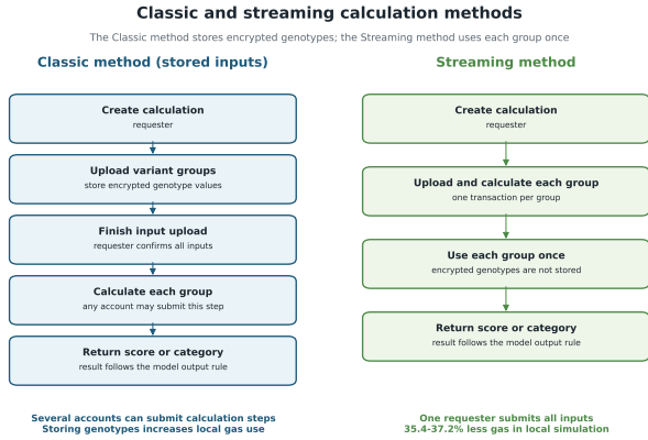
Figure 5: Calculation method comparison. The Classic method (stored inputs) uploads and stores SNPs before the score is calculated, so different parties can perform these steps. The Streaming method combines upload and calculation for one requester. Across the 100–5,000 variants evaluated in the local simulation, streaming used 35.4–37.2% less gas.
