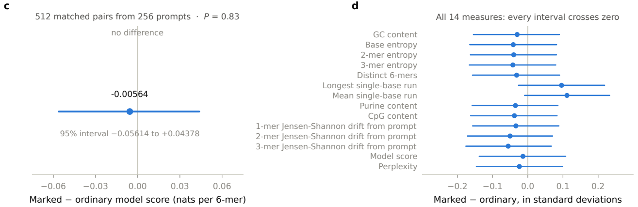
Figure 2: Model likelihood and sequence-quality proxies in the development cohort. a,c , Paired difference in model score between marked and ordinary continuations, over 512 matched pairs from 256 prompts. Positive values indicate lower model likelihood for marked continuations. The horizontal bar is the 95% interval from a bootstrap over prompts: -0.04426 to +0.05973 in Carbon ( P = 0.75 ) and -0.05614 to +0.04378 in GENERator ( P = 0.83 ). b,d , Paired differences for all 14 measures in standard deviations, with intervals in the same units. Every interval includes zero, and none of the 14 comparisons is significant after multiple-testing correction. Panels a,b show Carbon and panels c,d show GENERator.
