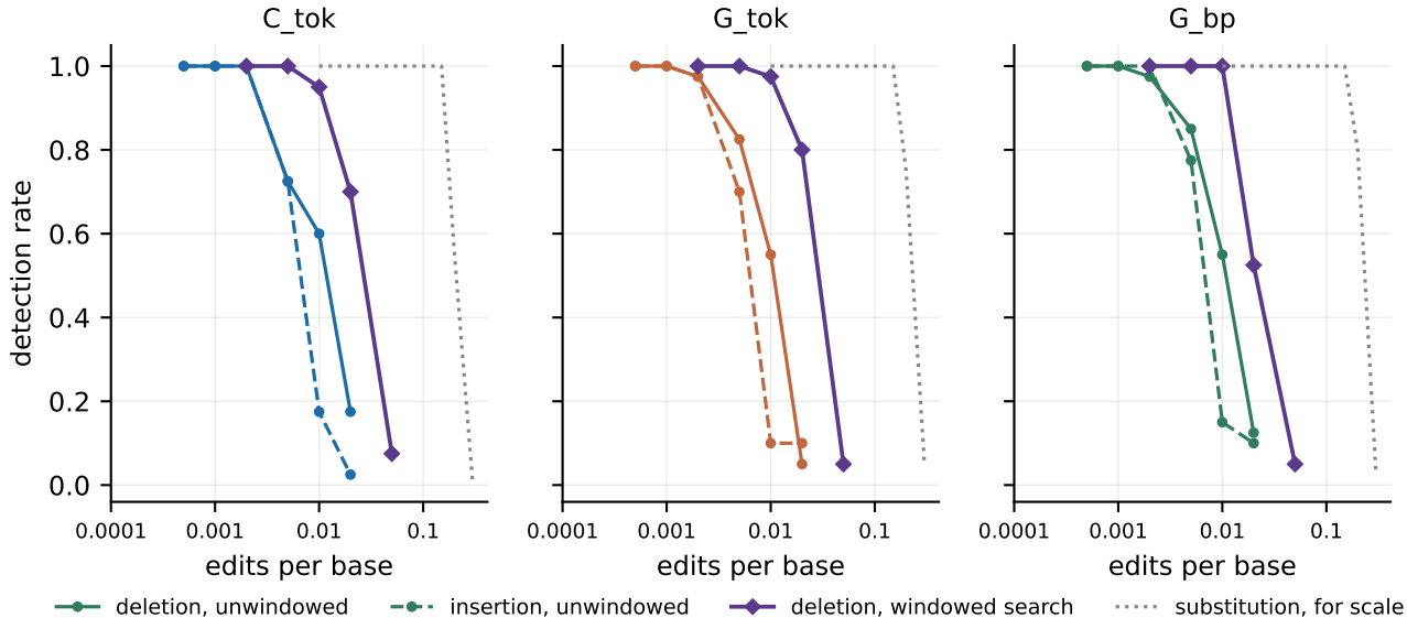
The synchronization wall, at 1,536 bases
