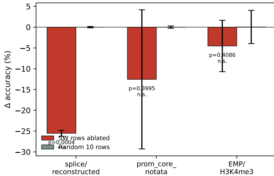
A. DNABERT-2 GUE \Delta acc — SW vs random control (3 seeds, mean \pm std)
