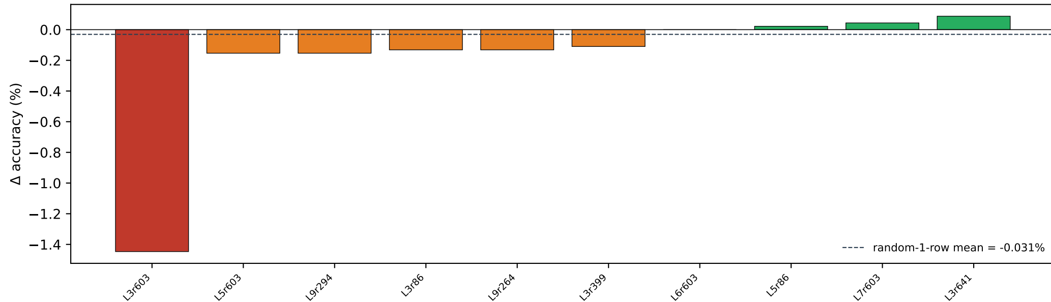
C. DNABERT-2 per-row \Delta acc on splice/reconstructed
