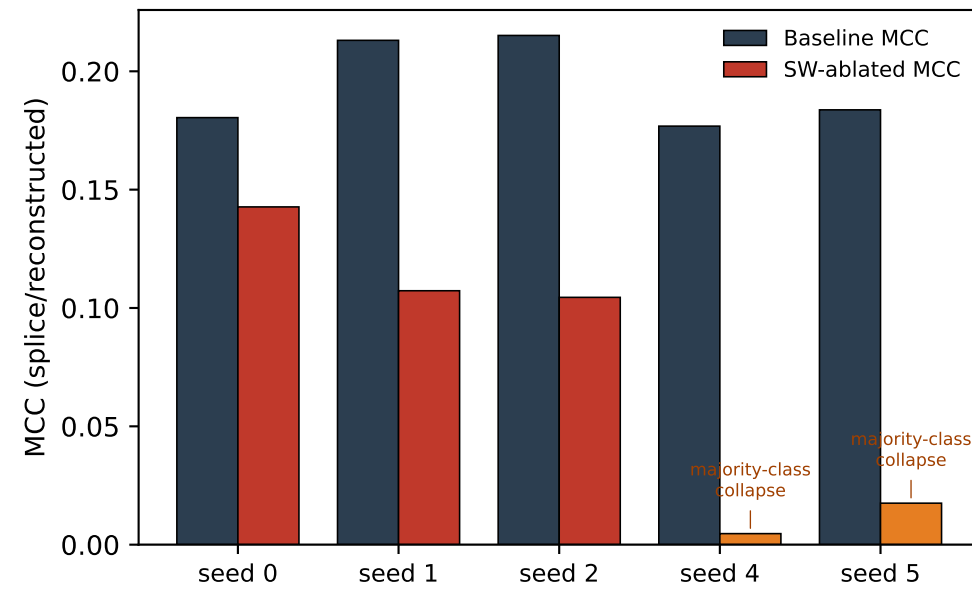
B. NTV3 splice — baseline vs SW-ablated MCC (5 seeds) \Delta MCC = -0.119 \pm 0.055 , t=-4.86 p=0.0083 , sign-neg 5/5
