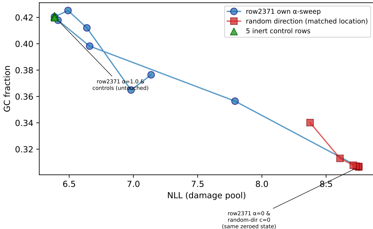
GENERator row 2371: GC vs. damage (NLL), all conditions
