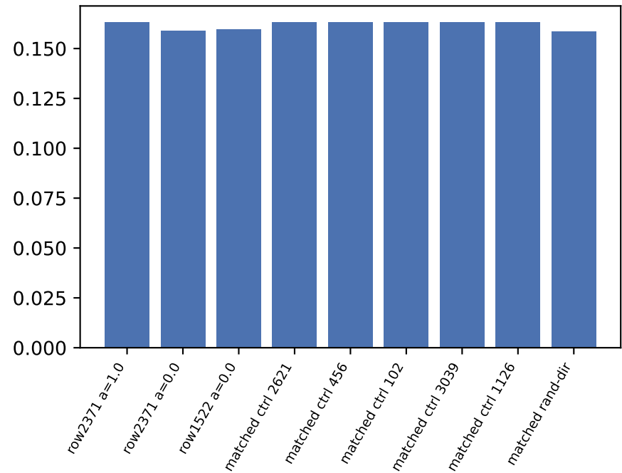
distinct3
