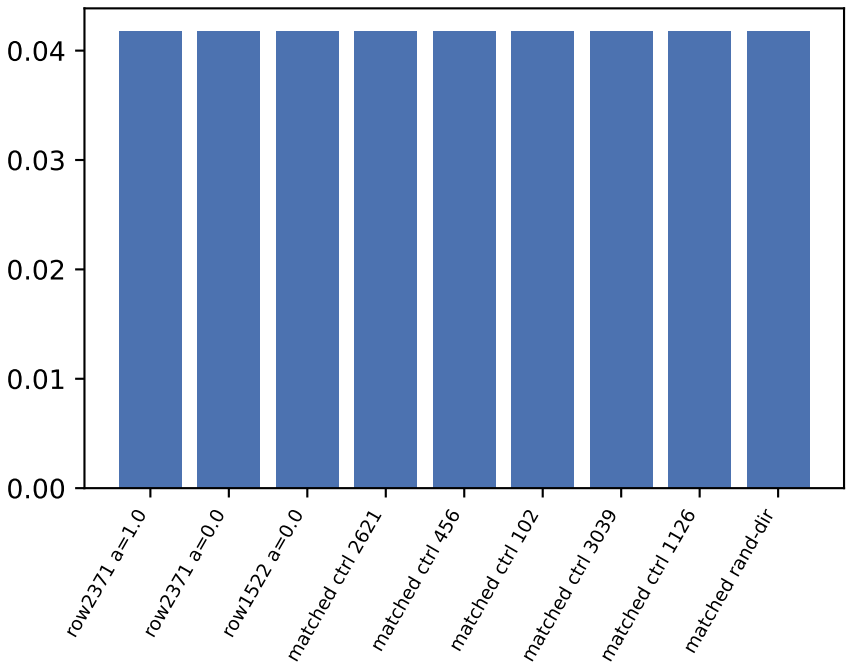
distinct2
