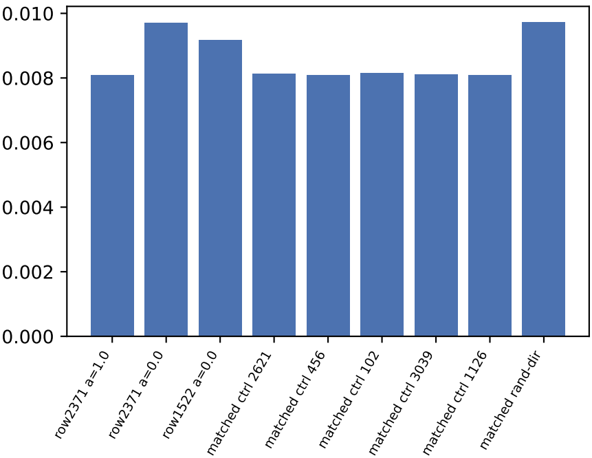
top6mer_share
