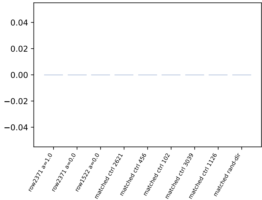
non_acgt_filter_rate
