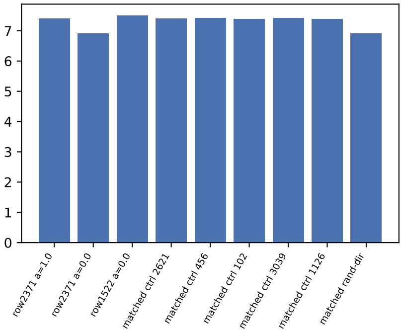
entropy
