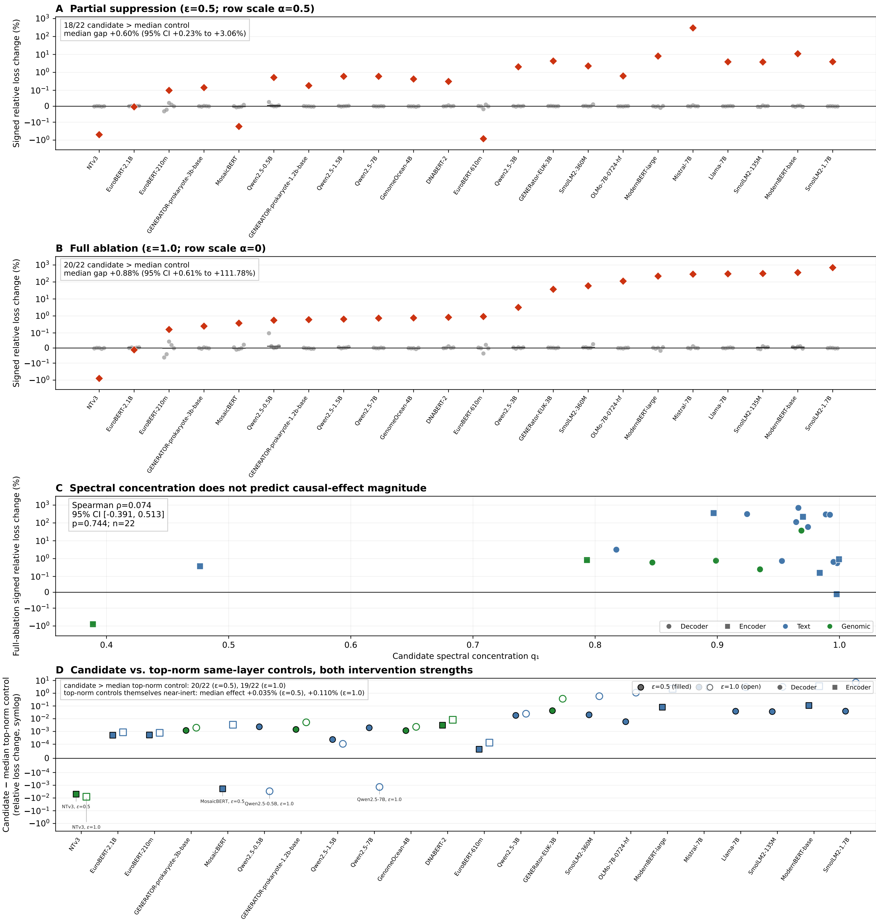
Figure 2 draft — functional criticality of frozen structural candidates across 22 models
