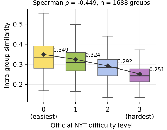
Figure 2: Intra-group embedding similarity (Eq. 1) against official NYT difficulty levels for 1,688 groups from 422 puzzles. Similarity decreases monotonically with official difficulty.
