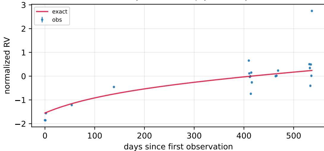
P=18.61 d, K=233.10 m/s, e=0.05 , n=26
