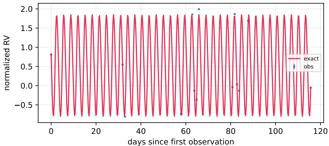
P=3.17 d, K=200.13 m/s, e=0.07 , n=14
