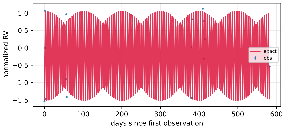
P=3.05 d, K=206.73 m/s, e=0.00 , n=30
