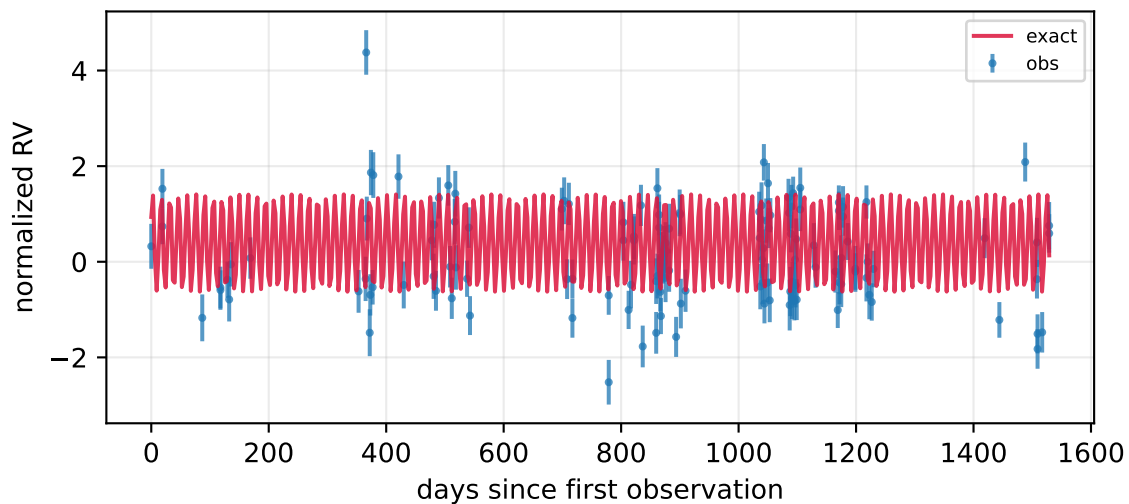
P=3.86 d, K=28.99 m/s, e=0.14 , n=137
