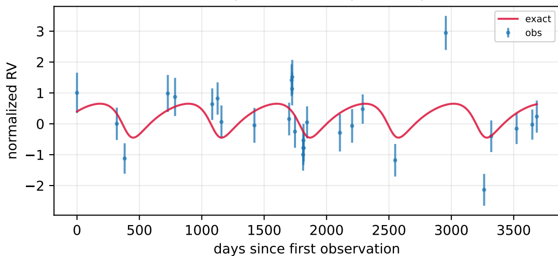
P=1242.41 d, K=256.19 m/s, e=0.10, n=21
