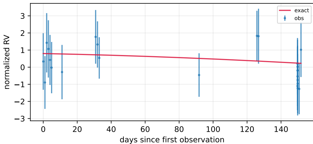
P=9.16 d, K=2.47 m/s, e=0.30 , n=12
