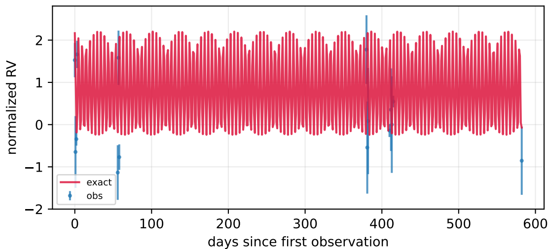
P=5.84 d, K=133.92 m/s, e=0.56 , n=30
