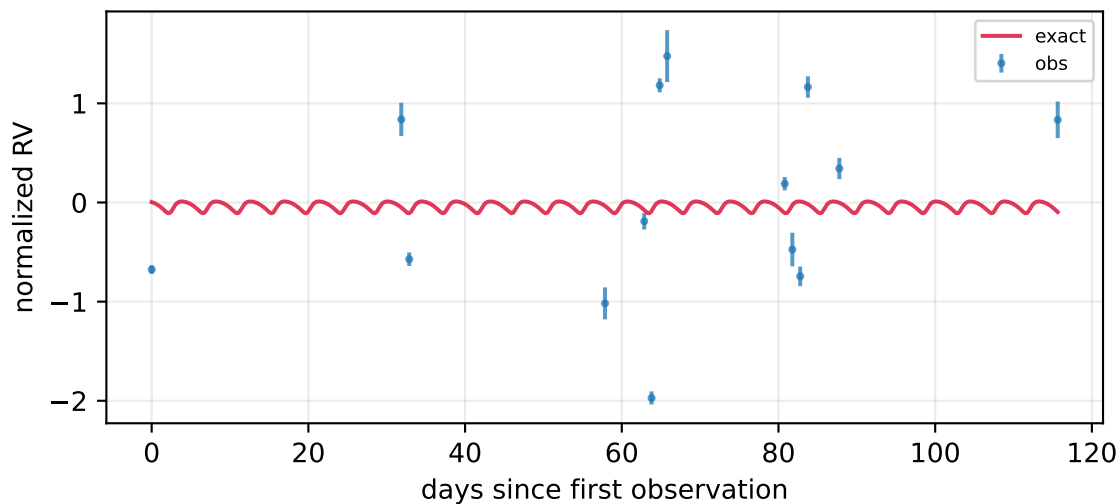
P=4.38 d, K=2.50 m/s, e=0.28 , n=14
