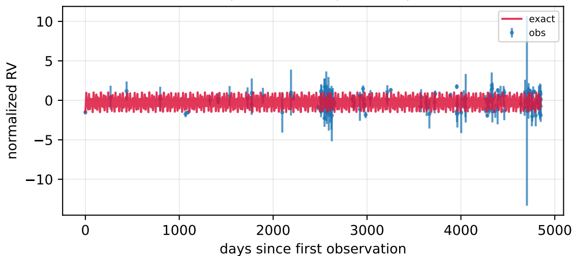
P=666.42 d, K=38.60 m/s, e=0.17, n=141
