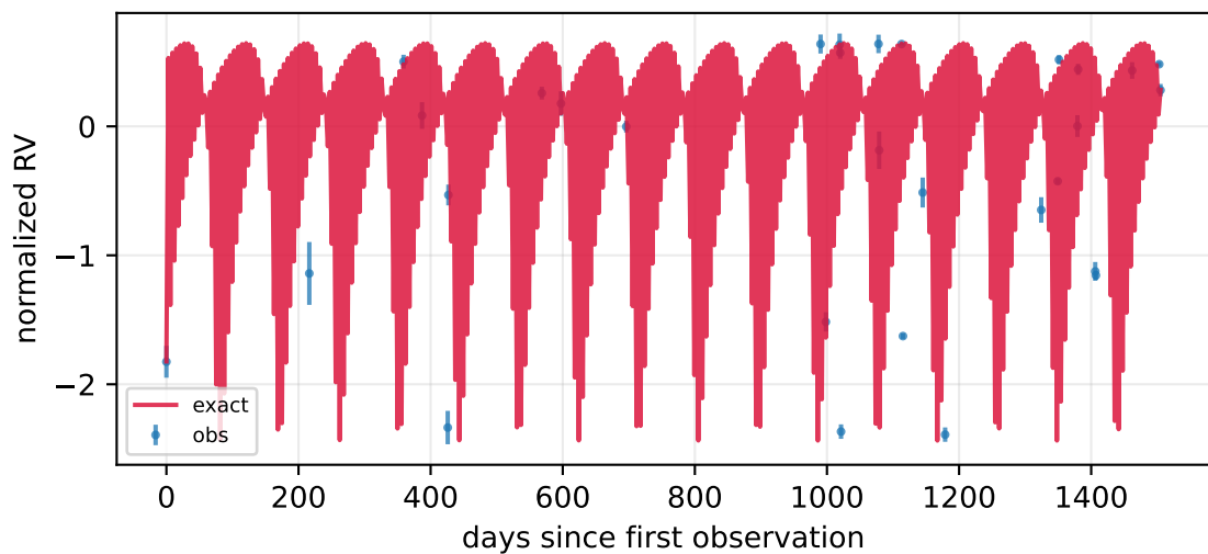
P=4.38 d, K=2.50 m/s, e=0.28 , n=14
