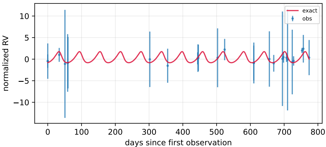
P=7.11 d, K=52.07 m/s, e=0.07 , n=137
