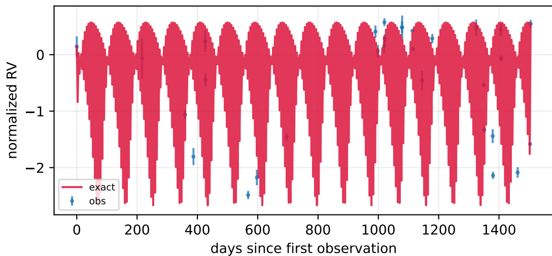
P=4.38 d, K=142.58 m/s, e=0.53 , n=14
