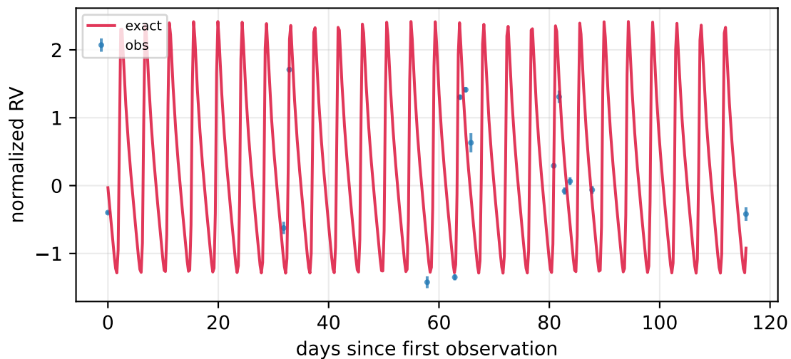
P=4.38 d, K=142.58 m/s, e=0.53 , n=14
