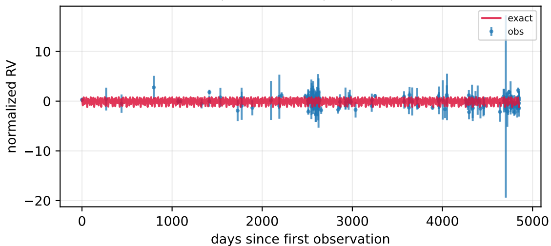
P=666.42 d, K=263.05 m/s, e=0.03, n=141
