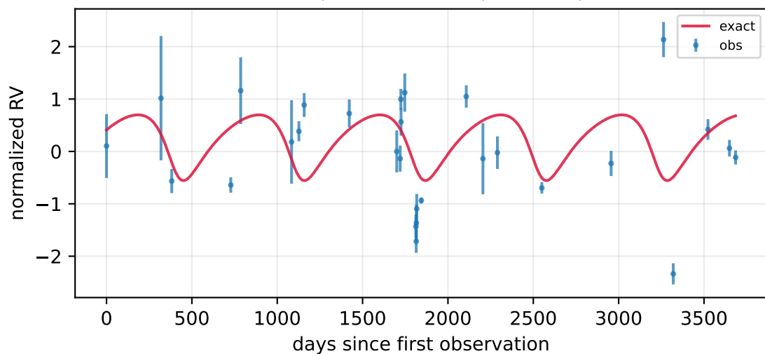
P=1242.41 d, K=256.19 m/s, e=0.10 , n=21
