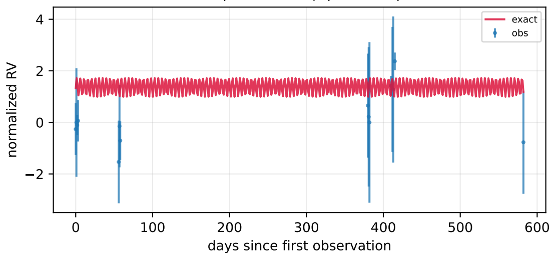
P=5.84 d, K=96.57 m/s, e=0.40 , n=30
