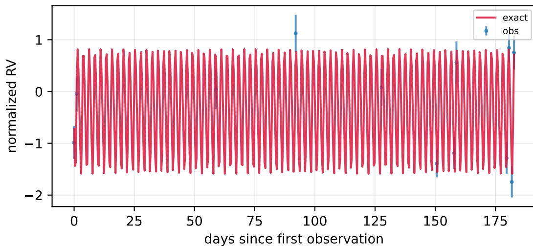
P=2.39 d, K=16.19 m/s, e=0.20 , n=12
