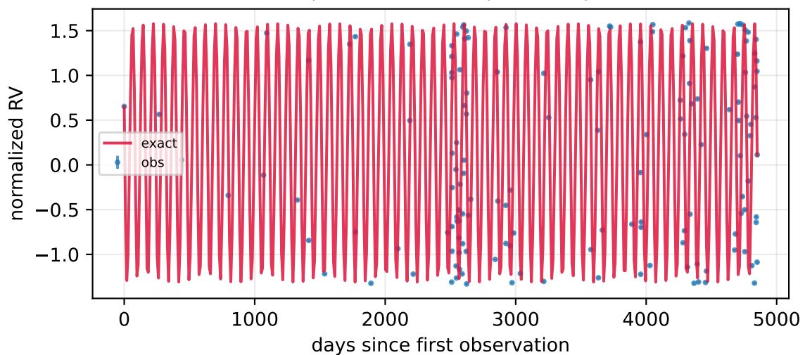
P=1111.78 d, K=68.70 m/s, e=0.11 , n=141
