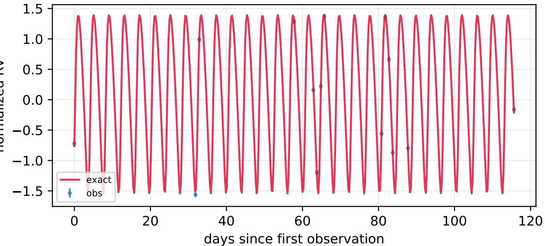
P=4.04 d, K=58.56 m/s, e=0.25 , n=14
