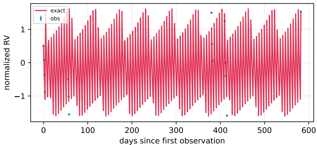
P=3.48 d, K=99.39 m/s, e=0.35 , n=30
