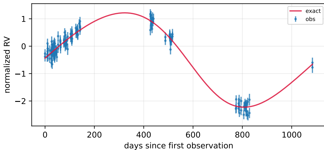
P=1318.24 d, K=161.16 m/s, e=0.54 , n=24
