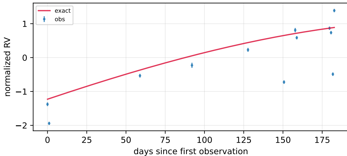
P=4.10 d, K=74.53 m/s, e=0.16 , n=11
