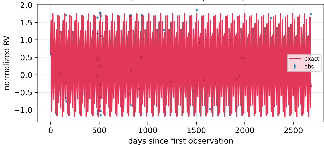
P=3.17 d, K=200.13 m/s, e=0.07 , n=50
