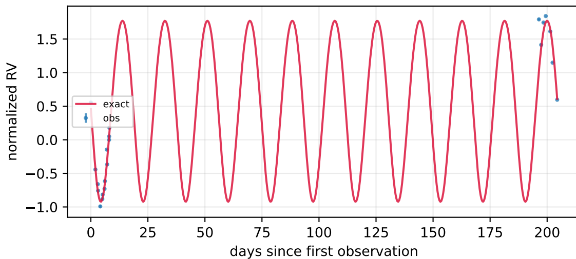
P=3.86 d, K=28.99 m/s, e=0.14 , n=35
