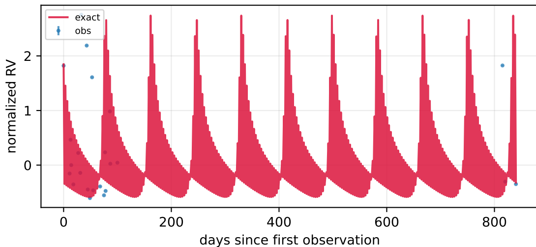
P=550.42 d, K=406.73 m/s, e=0.78 , n=11
