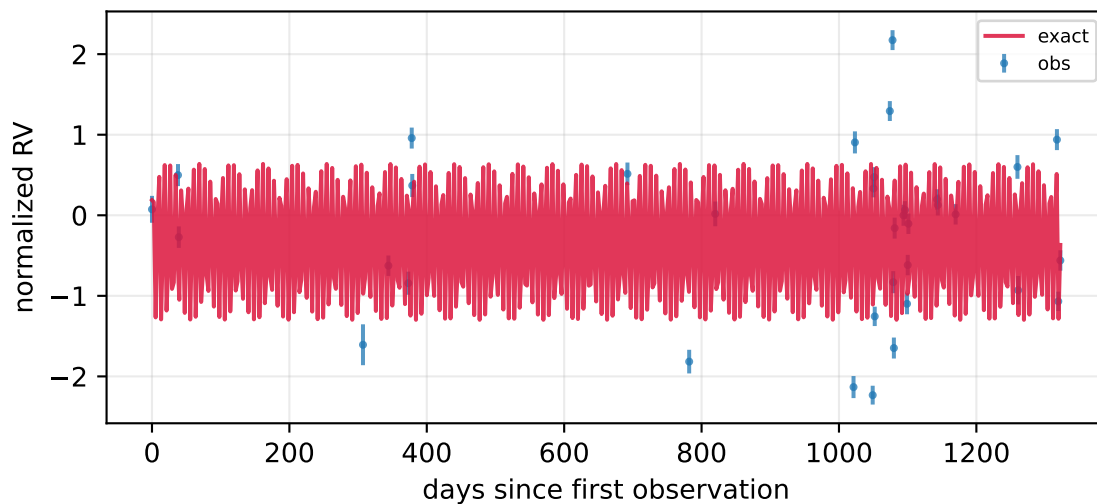
P=3.86 d, K=28.99 m/s, e=0.14 , n=35
