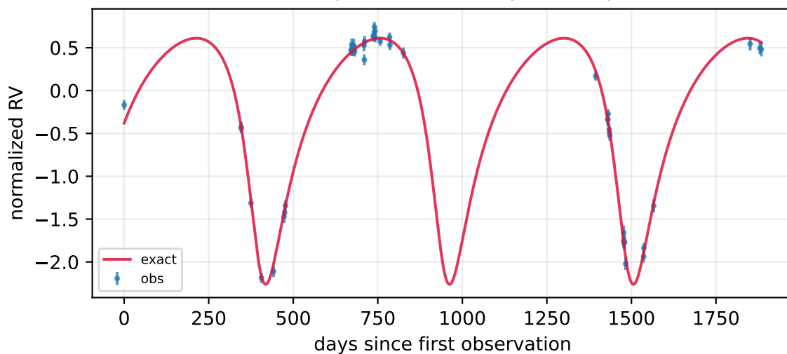
P=981.88 d, K=98.37 m/s, e=0.71 , n=49
