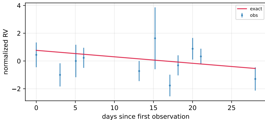
P=1259.51 d, K=126.60 m/s, e=0.05 , n=12
