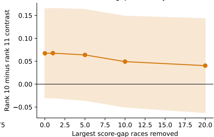
Extreme-gap sensitivity
