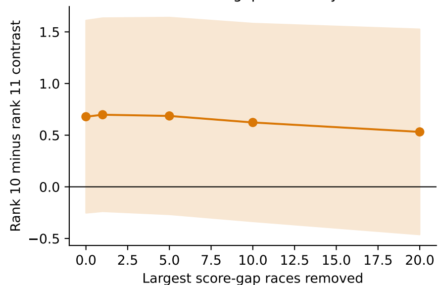
Extreme-gap sensitivity
