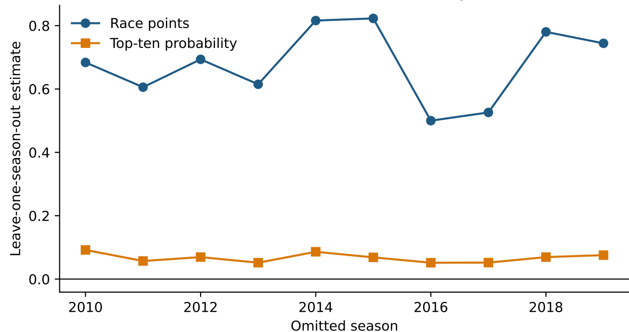
Leave-one-season-out sensitivity
