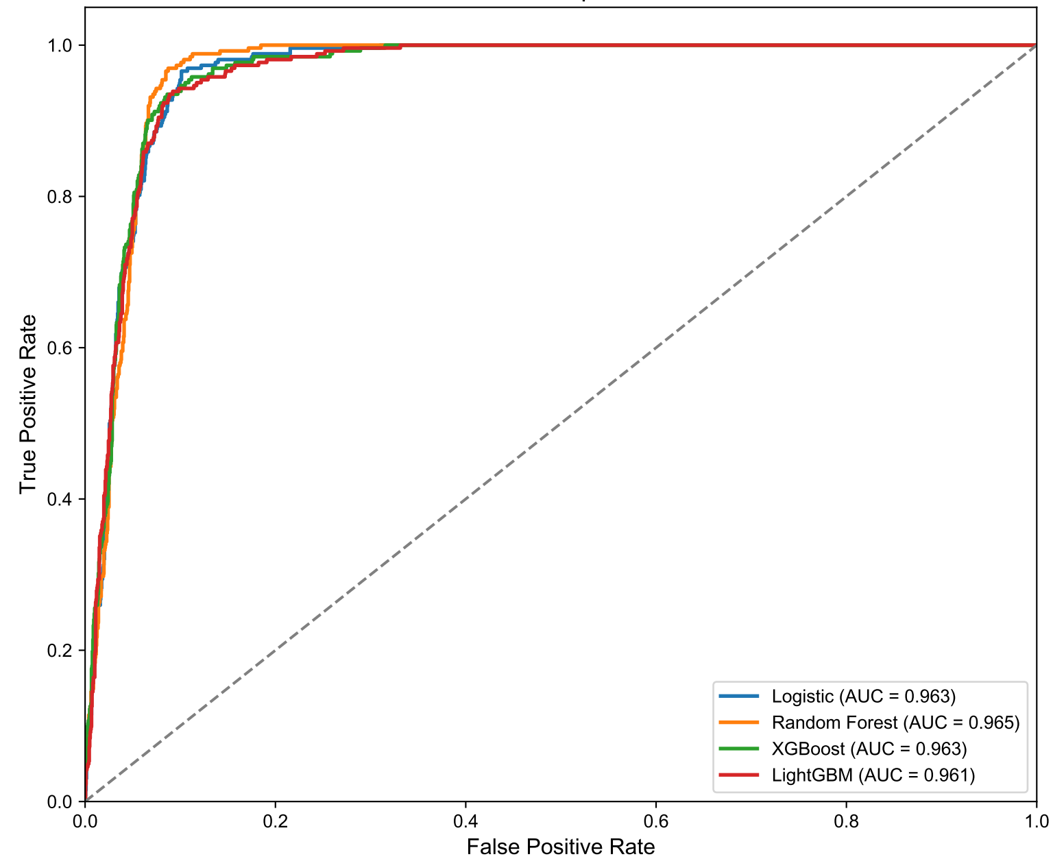
ROC Curve Comparison Chart
