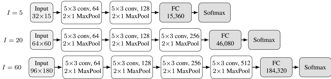
Figure 2: Horizon-specific CNN backbones (cf. Figure 2 of the original paper). Each rectangle is one block: 5 \times 3 convolution (with the channel width shown), LeakyReLU, batch normalisation, and 2 \times 1 max pooling. Stride and dilation for I = 20 and I = 60 are in Table 5. FC widths 15,360 / 46,080 / 184,320 match our implementation.
