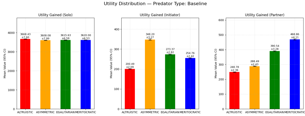
Figure 4.4: Baseline Predator - Utility Distribution (Heterogeneous, Normal Synergy).
