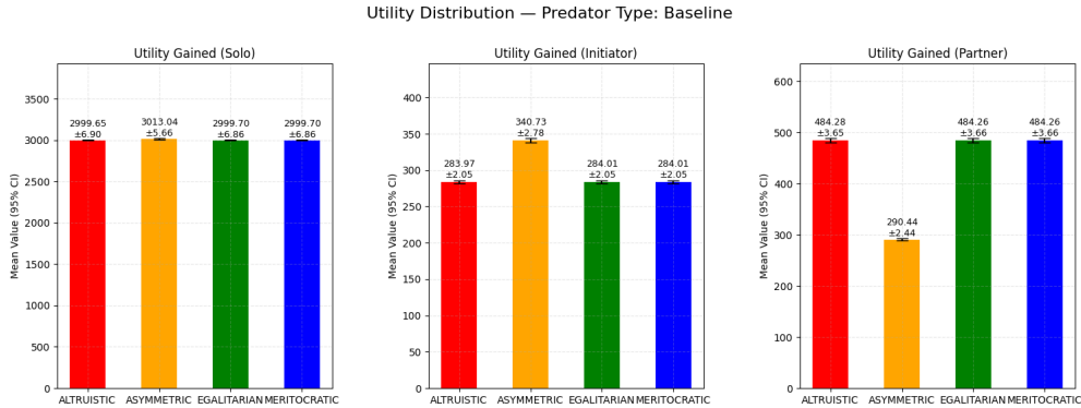
Figure 4.2: Baseline Predator - Utility Distribution (Homogeneous, Normal Synergy).
