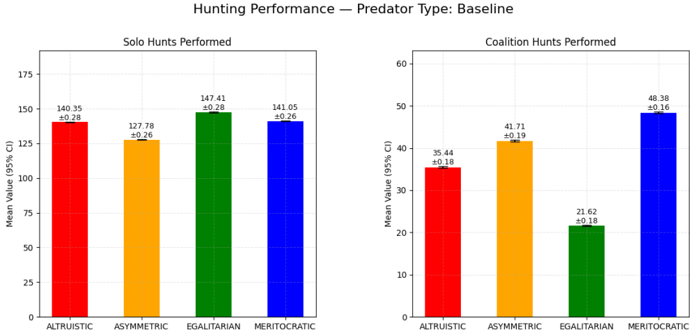
Figure 4.11: Baseline Predator - Hunting Performance (Heterogeneous, High Synergy).
