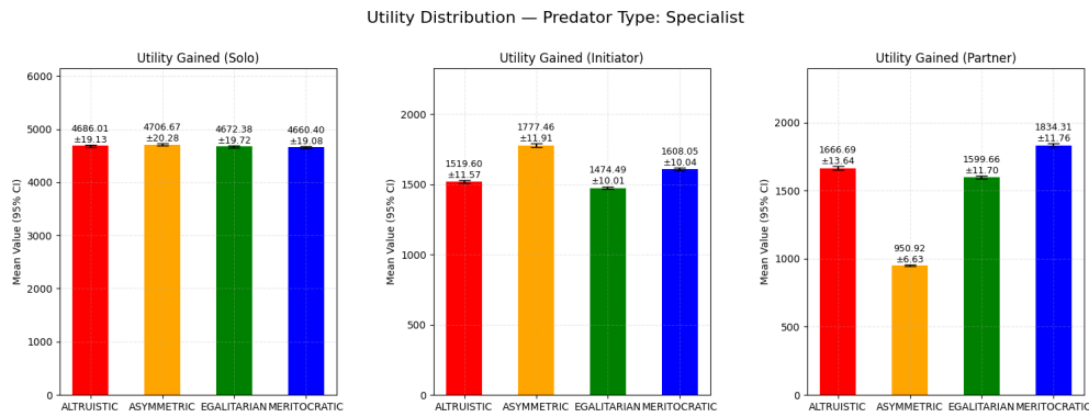
Figure 4.6: Specialist Predator - Utility Distribution (Heterogeneous, Normal Synergy).
