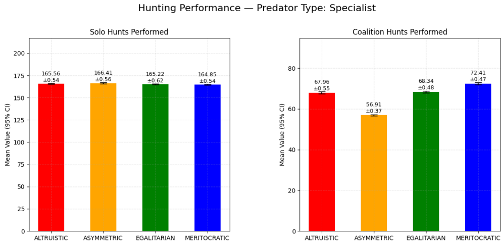
Figure 4.5: Specialist Predator - Hunting Performance (Heterogeneous, Normal Synergy).
