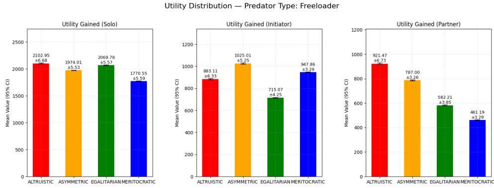
Figure 4.16: Freeloader Predator - Utility Distribution (Heterogeneous, High Synergy).
