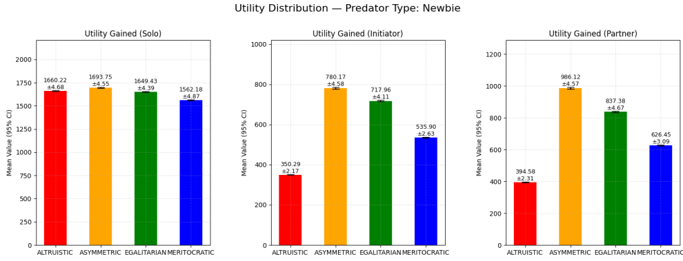
Figure 4.18: Newbie Predator - Utility Distribution (Heterogeneous, High Synergy).
