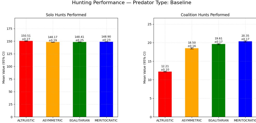
Figure 4.3: Baseline Predator - Hunting Performance (Heterogeneous, Normal Synergy).
