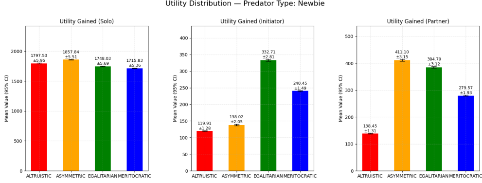
Figure 4.10: Newbie Predator - Utility Distribution (Heterogeneous, Normal Synergy).
