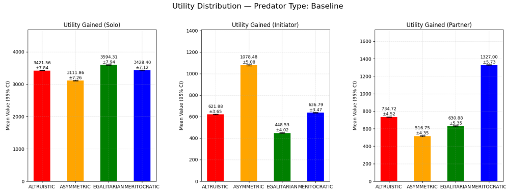
Figure 4.12: Baseline Predator - Utility Distribution (Heterogeneous, High Synergy).
