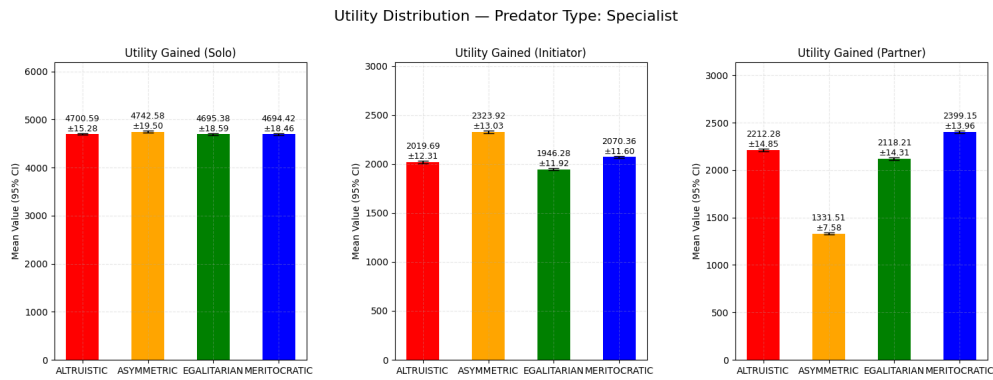
Figure 4.14: Specialist Predator - Utility Distribution (Heterogeneous, High Synergy).
