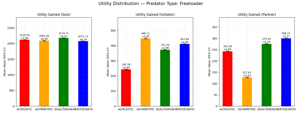
Figure 4.8: Freeloader Predator - Utility Distribution (Heterogeneous, Normal Synergy).
