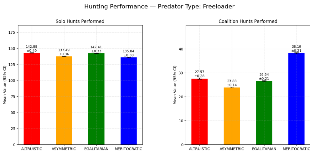
Figure 4.7: Freeloader Predator - Hunting Performance (Heterogeneous, Normal Synergy).
