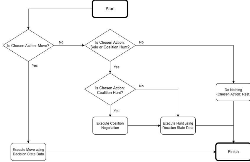
Figure 3.4: Predator Execution Cycle Flowchart.
