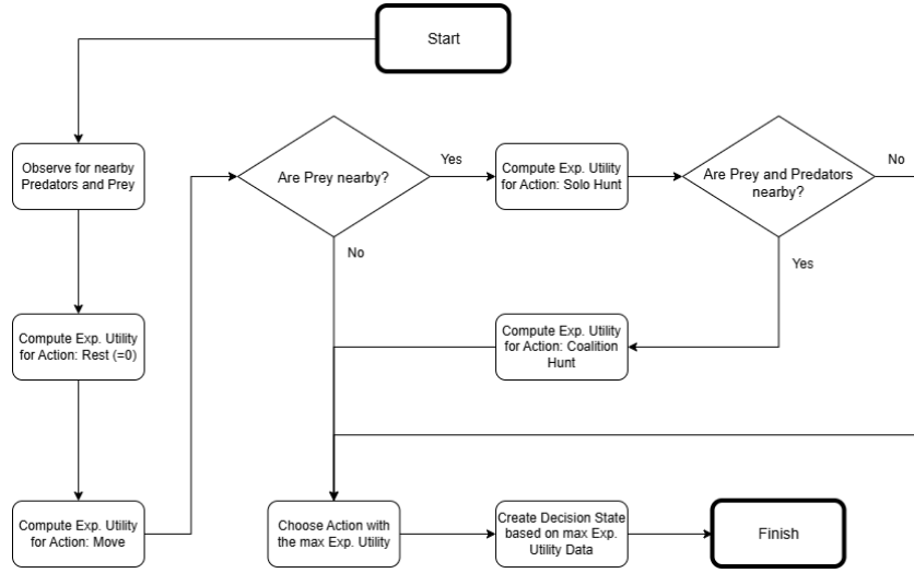
Figure 3.3: Predator Decision Cycle Flowchart.
