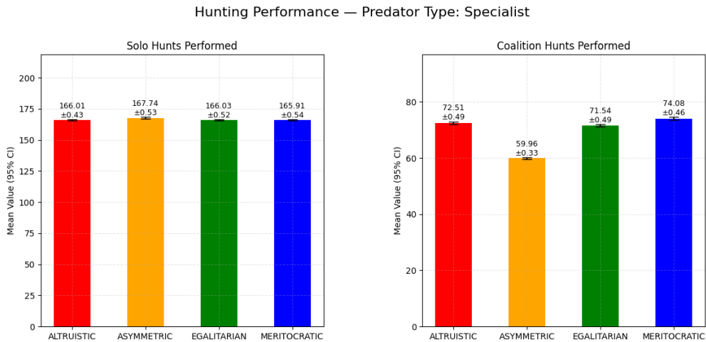
Figure 4.13: Specialist Predator - Hunting Performance (Heterogeneous, High Synergy).
