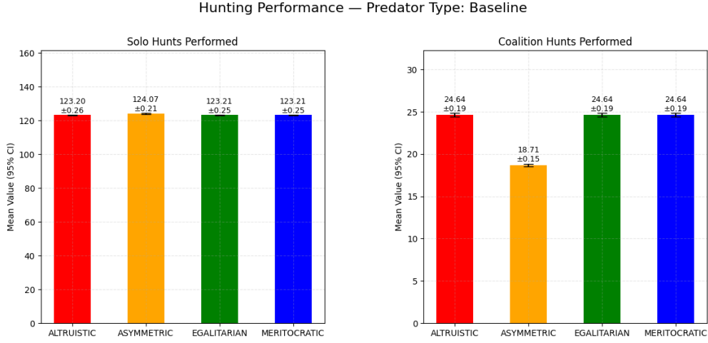
Figure 4.1: Baseline Predator - Hunting Performance (Homogeneous, Normal Synergy).
