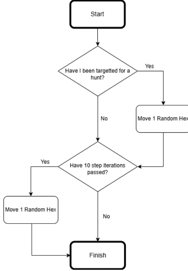
Figure 3.2: Prey Action Cycle Flowchart.
