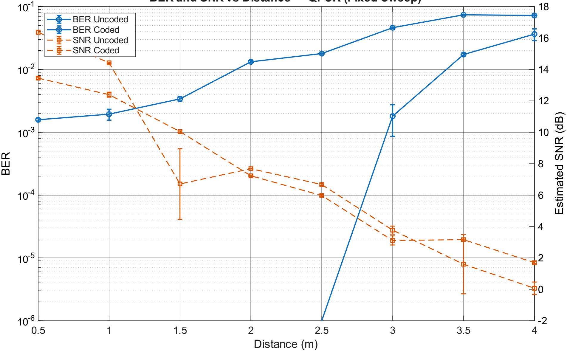
BER and SNR vs Distance — QPSK (Fixed Sweep)
