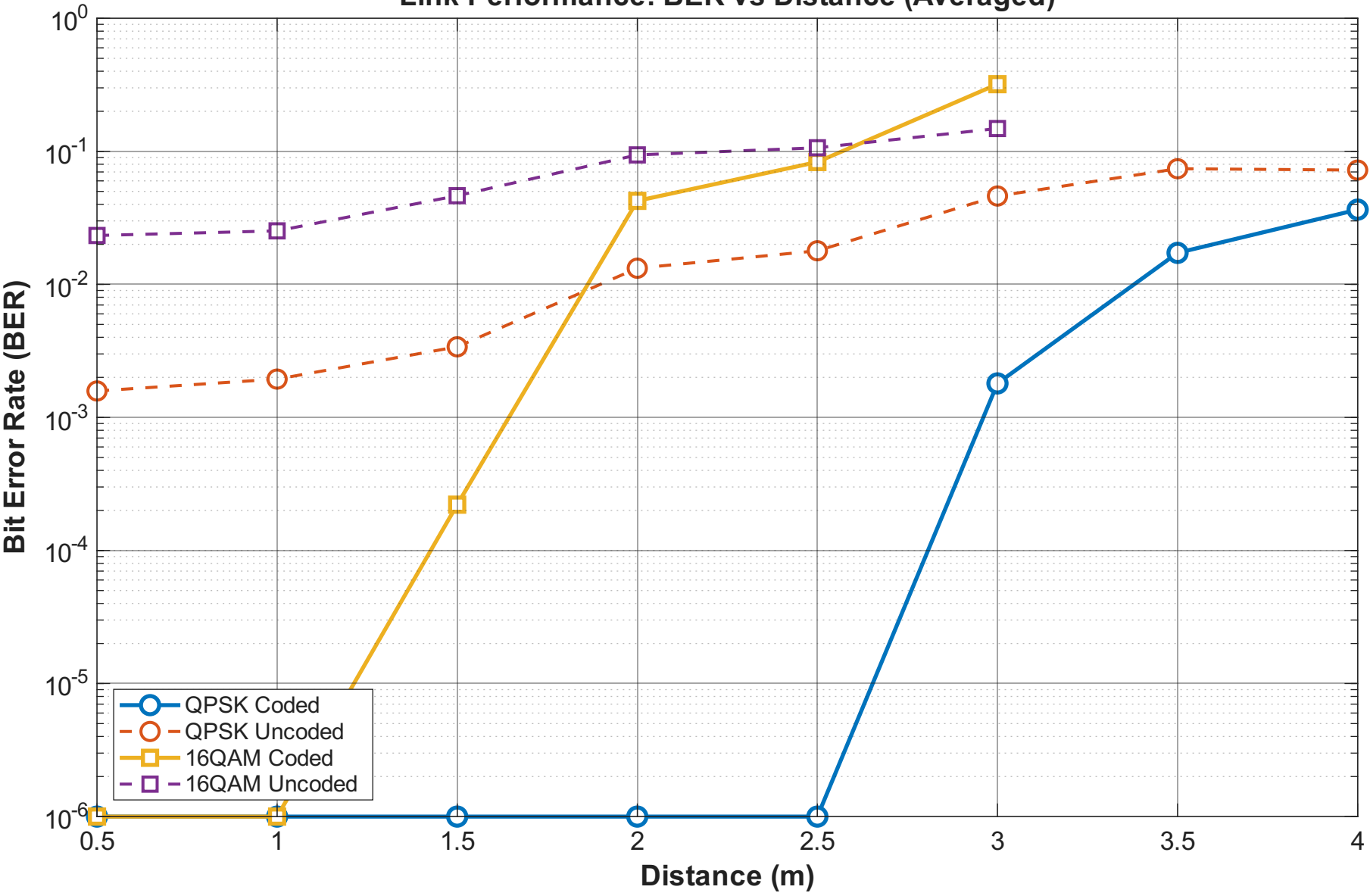
Link Performance: BER vs Distance (Averaged)
